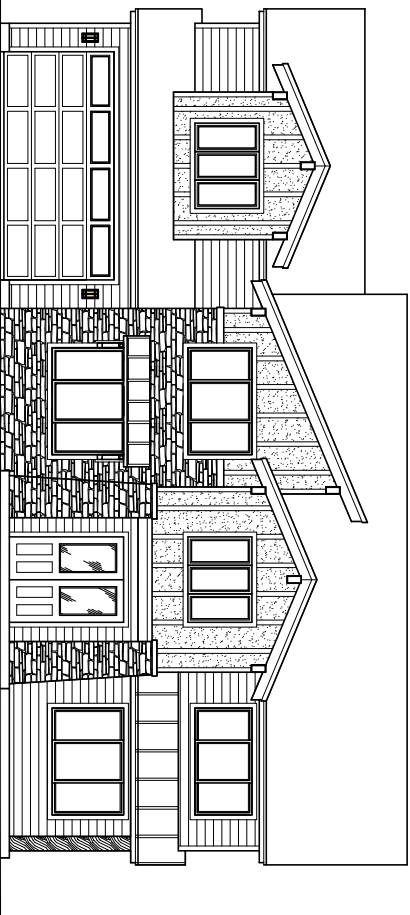
Plan 3288 Elevation 'C'
