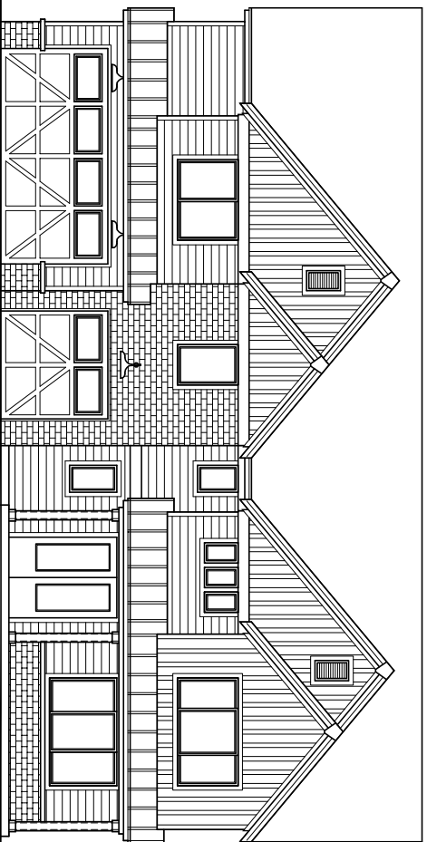
Plan 3542 Elevation 'A'
